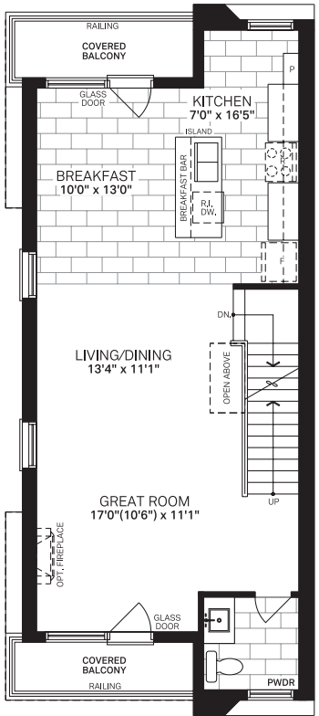
MAIN FLOOR PLAN
